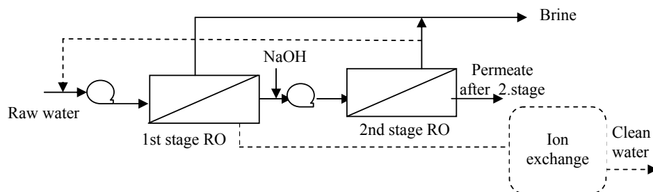
Fig. 1. Two stage RO system for boron removal
